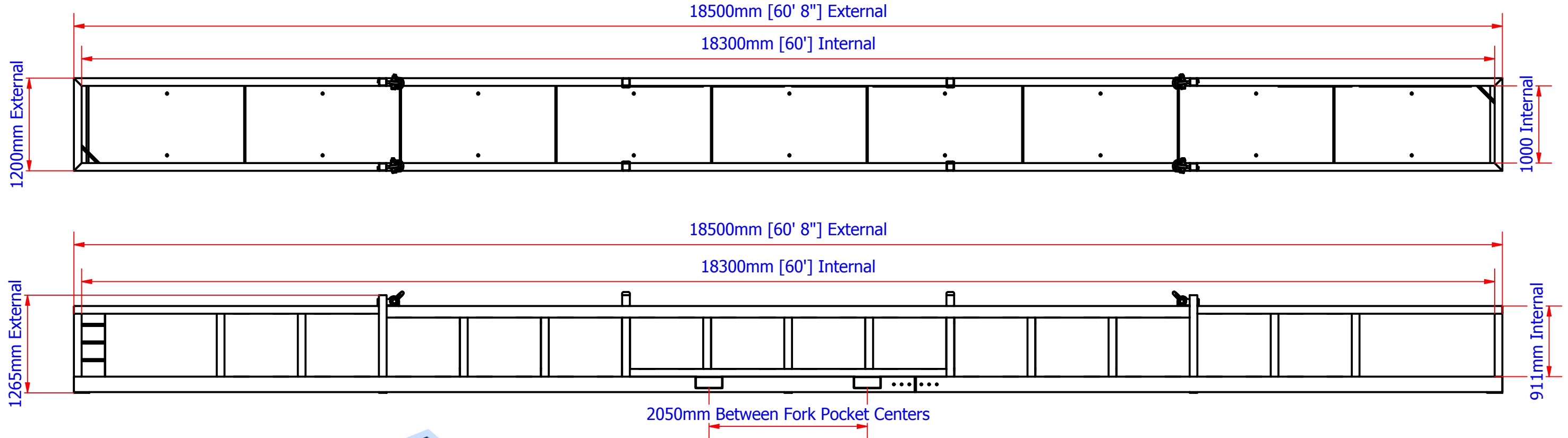
Internal Lashing Bar System
