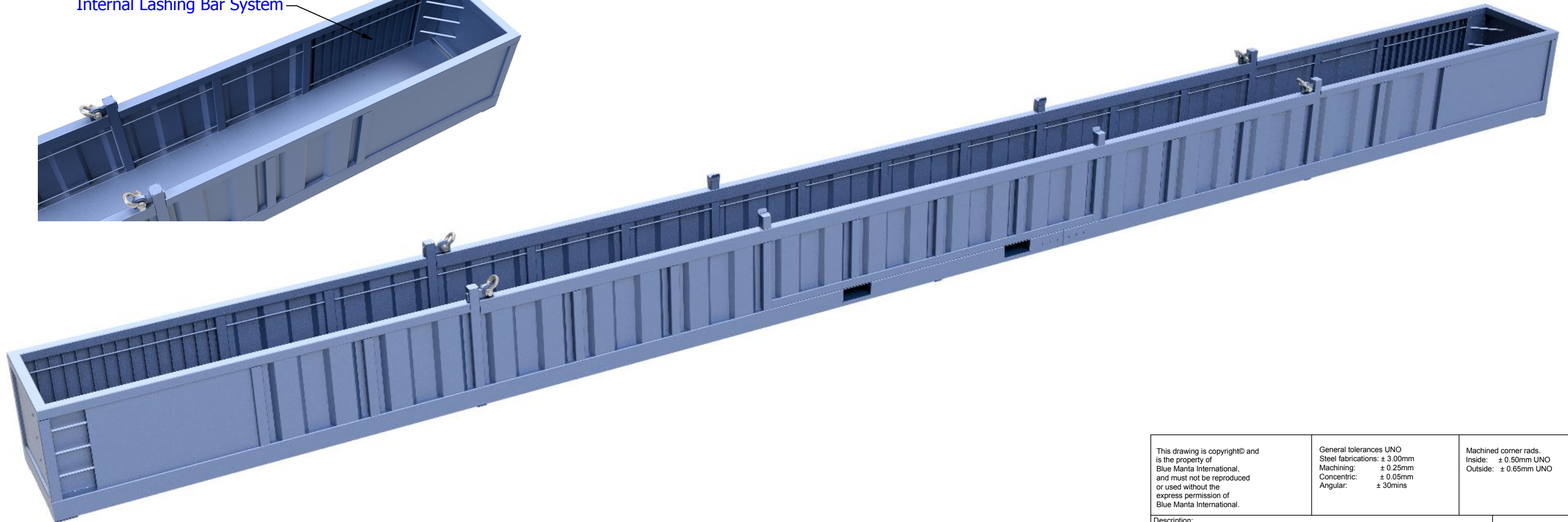
Internal Lashing Bar System
